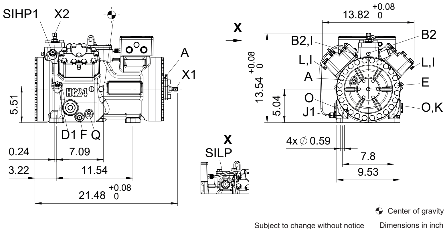
Dimensions and connections with accessories shut-off valves
