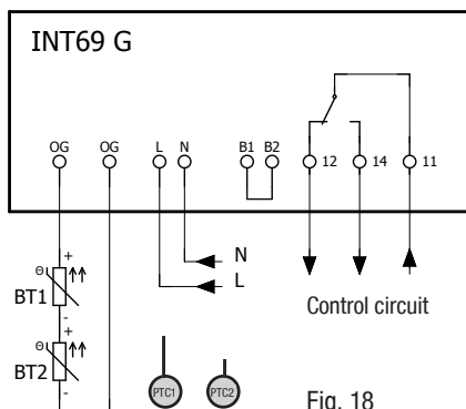
Fig. 18 Terminal box
