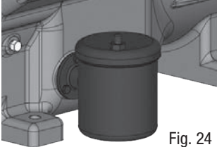
Fig. 24 Mechanical oil level regulator at the "O" connection
