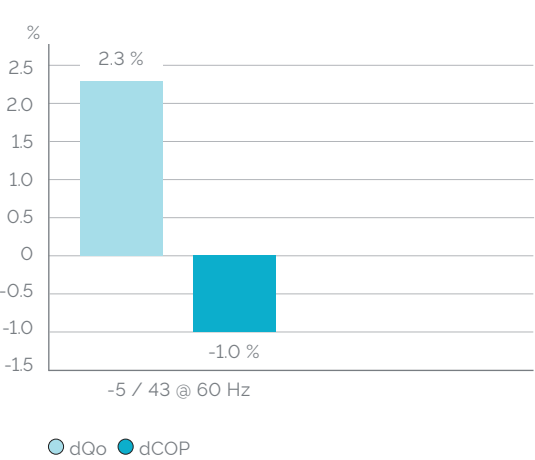
Capacity data SHG44e/665-4 SL Refrigerant: R134A
