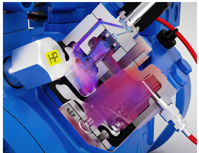
Capacity regulator active (solenoid energized): Operation of the cylinder bank in partial load (bypass) (digital or conventional).
